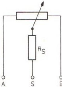
Potentiometer R = 25 \text{ k}\Omega R_S = 330 \Omega P = 1/4 \text{ W/lin}
