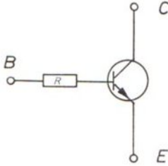
Transistor BC 108 A R = \text{Schutzwiderstand } (1 \text{ k}\Omega)
