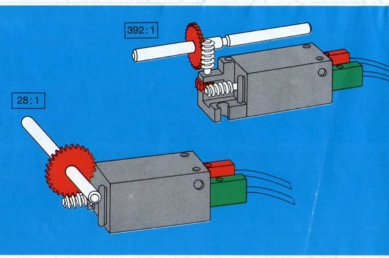
mini-motor with gearbox
